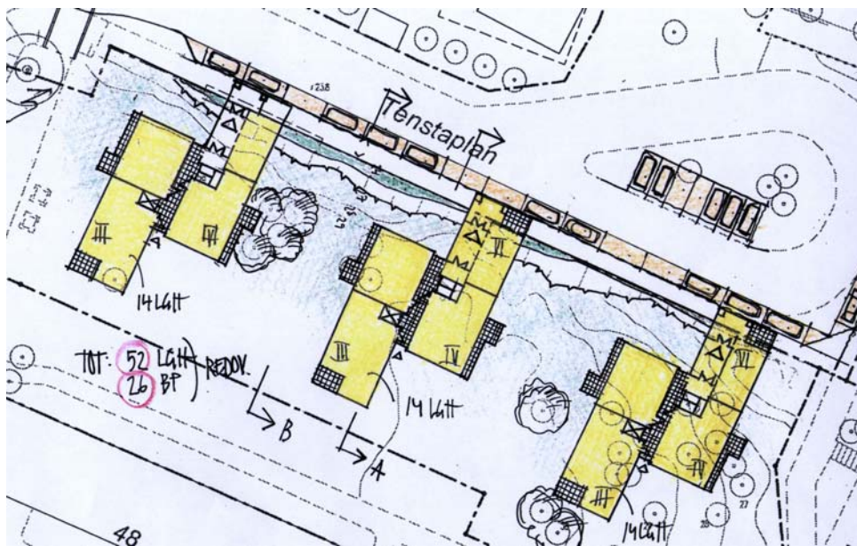
Situationsplan
